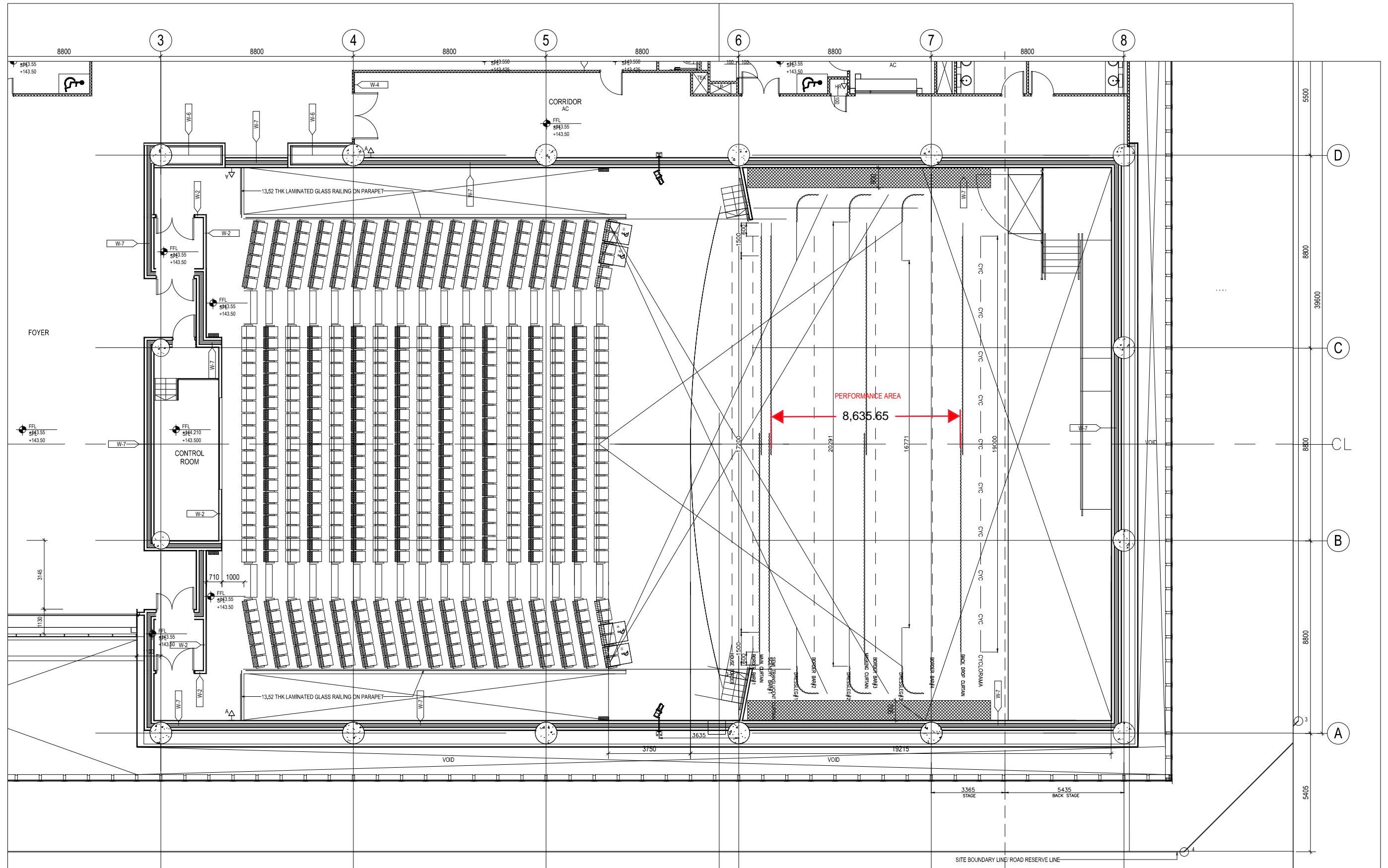
AUDITORIUM STAGE PLAN SCALE: NOT TO SCALE
